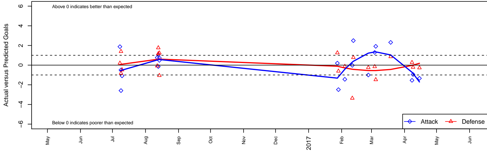
NEU White B00 Dots are actual minus expected GF (blue circles) and GA (red triangles). Blue line is smoothed change in attack strength. Red is smoothed change in defense strength.
